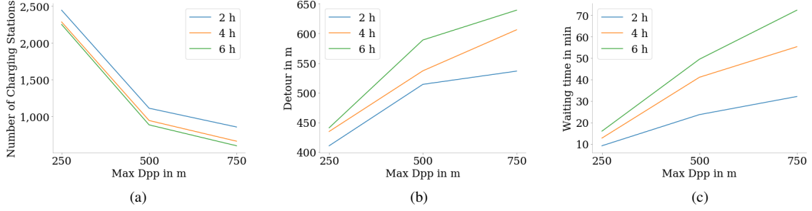
Fig. 3: (a) Number of CSs, (b) detour, and (c) waiting time for different d_{pp,max} and \tilde{\sigma}_{max} scenarios.
