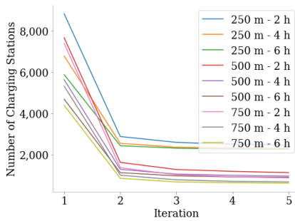
Fig. 2: Number of CSs over iteration for different consolidation parameters d_{pp,max} and \tilde{\sigma}_{max} .
